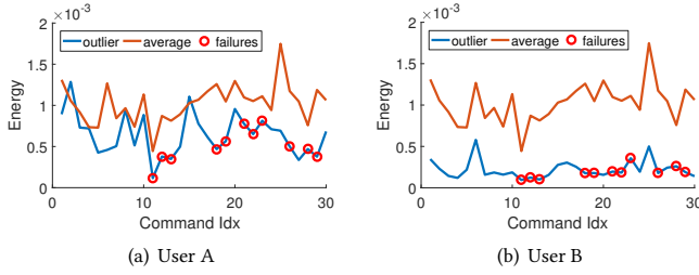
Figure 11: The energy levels of the outlier users (in Fig. 10(c)) compared to average users. The circles represent commands of the outlier users that VAuth fails to match.
