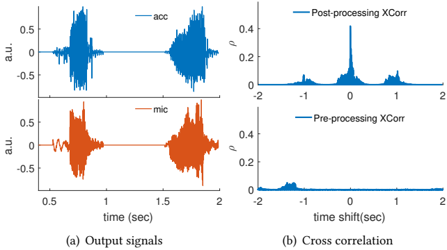
Figure 8: Matching decision stage of VAuth's matching.
