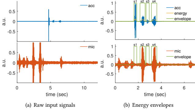
Figure 6: Pre-processing stage of VAuth’s matching.
