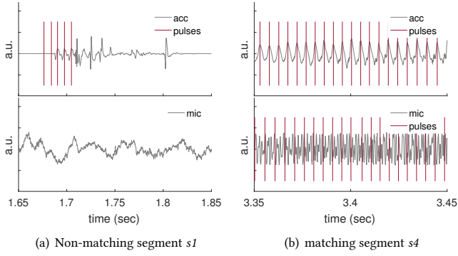
Figure 7: Per-segment analysis stage of VAuth.
