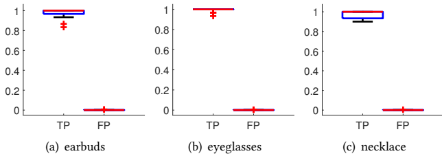
Figure 12: The detection accuracy of VAuth for the 18 users in the moving position.
