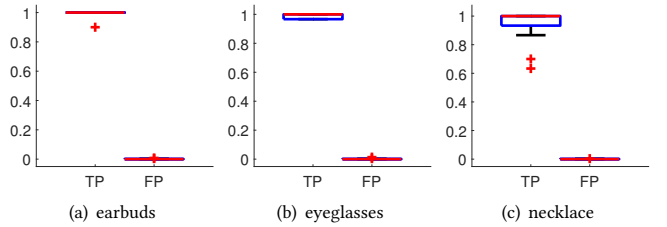
Figure 10: The detection accuracy of VAuth for the 18 users in the still position.
